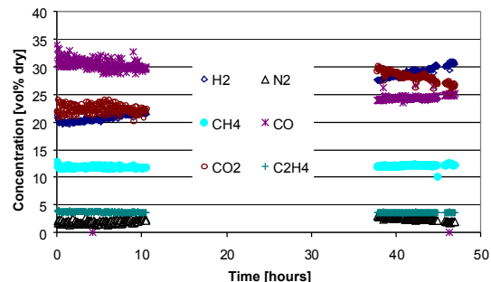
Figure 2: MILENA raw gas composition
