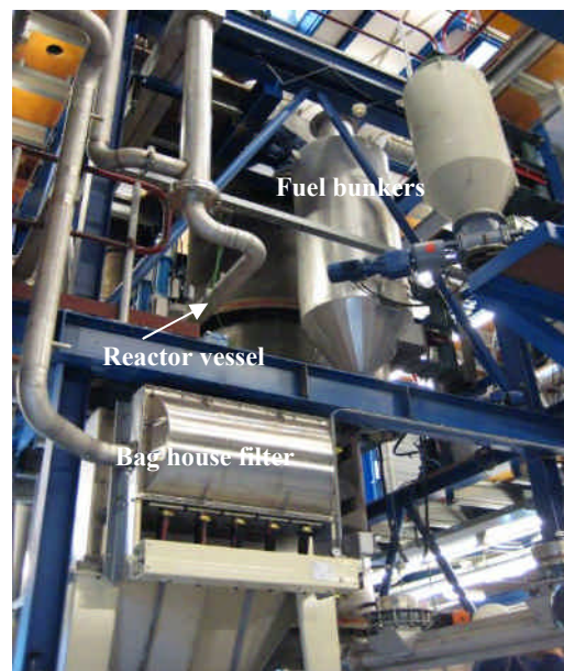
Figure 5: MILENA pilot nearly finished
