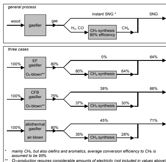
Figure 1. Green Gas production efficiencies for different gasification technologies, EF: entrained flow, CFB: circulating fluidised bed
